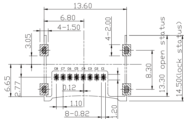
Recommended PCB Layout (PCB TOLERANCE±0.05)
