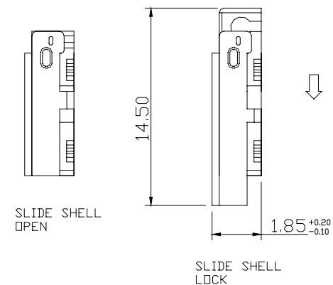
MICRO SD CARD(T-Flash)
